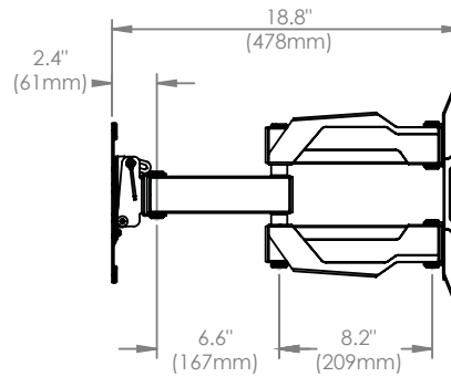
SIDE VIEW (EXTENDED)
